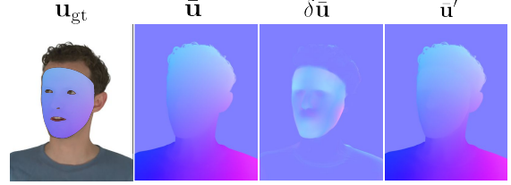
Figure 4. UV-space predictions. Given a ground truth per-pixel UV-coordinates \mathbf{u}_{\text{gt}} , our model is supervised to match the expectation of warped coordinates \bar{\mathbf{u}}' to the ground truth. We visualize the expectations of the spherically mapped coordinates \bar{\mathbf{u}} and the warps \delta \bar{\mathbf{u}} for reference.
