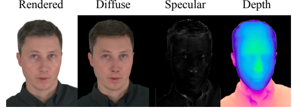
Figure 3. Radiance decomposition. During training, the radiance is modeled using spherical harmonics coefficients, which can be decomposed into diffuse (view-independent) and specular (view-dependent) components. The appearance can be exported as just diffuse or both diffuse and specular texture images.
